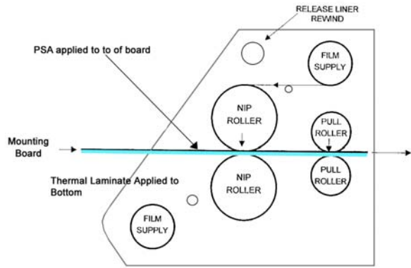
Typical Roll Laminator Configuration
